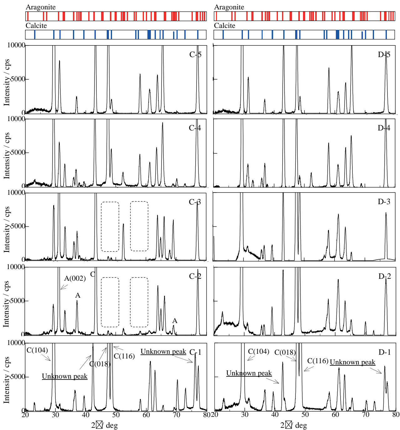
Fig.9 XRD profiles of Mizuhopecten yessoensis (Right shell)
