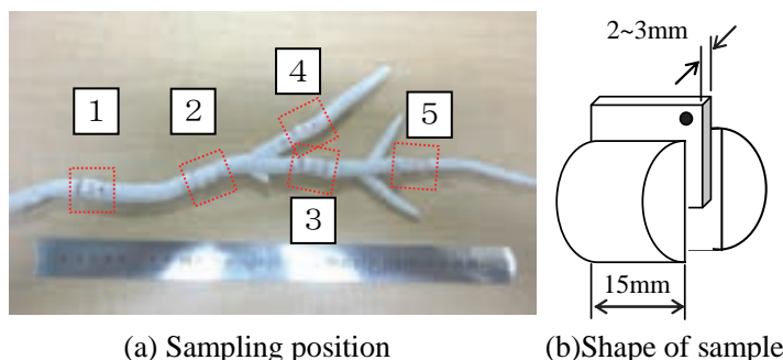
Fig.2 Detail of XRD measurement sample
