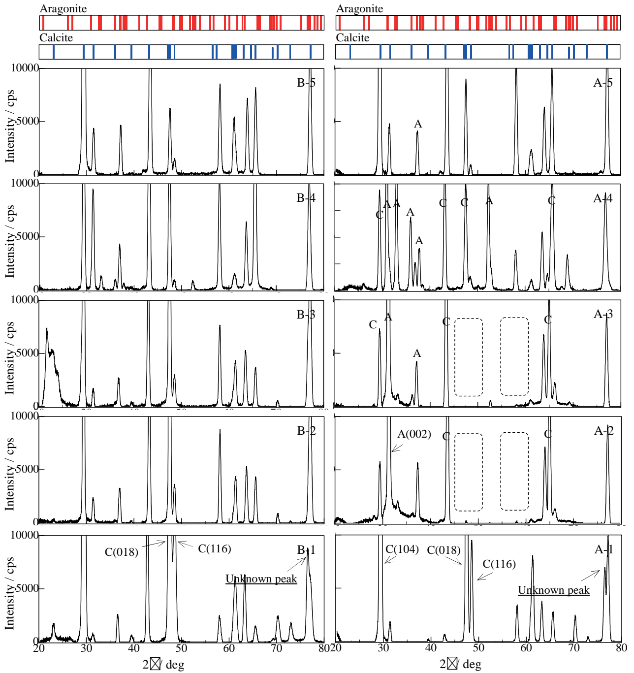
Fig.8 XRD profiles of Mizuhopecten yessoensis (Left shell)
